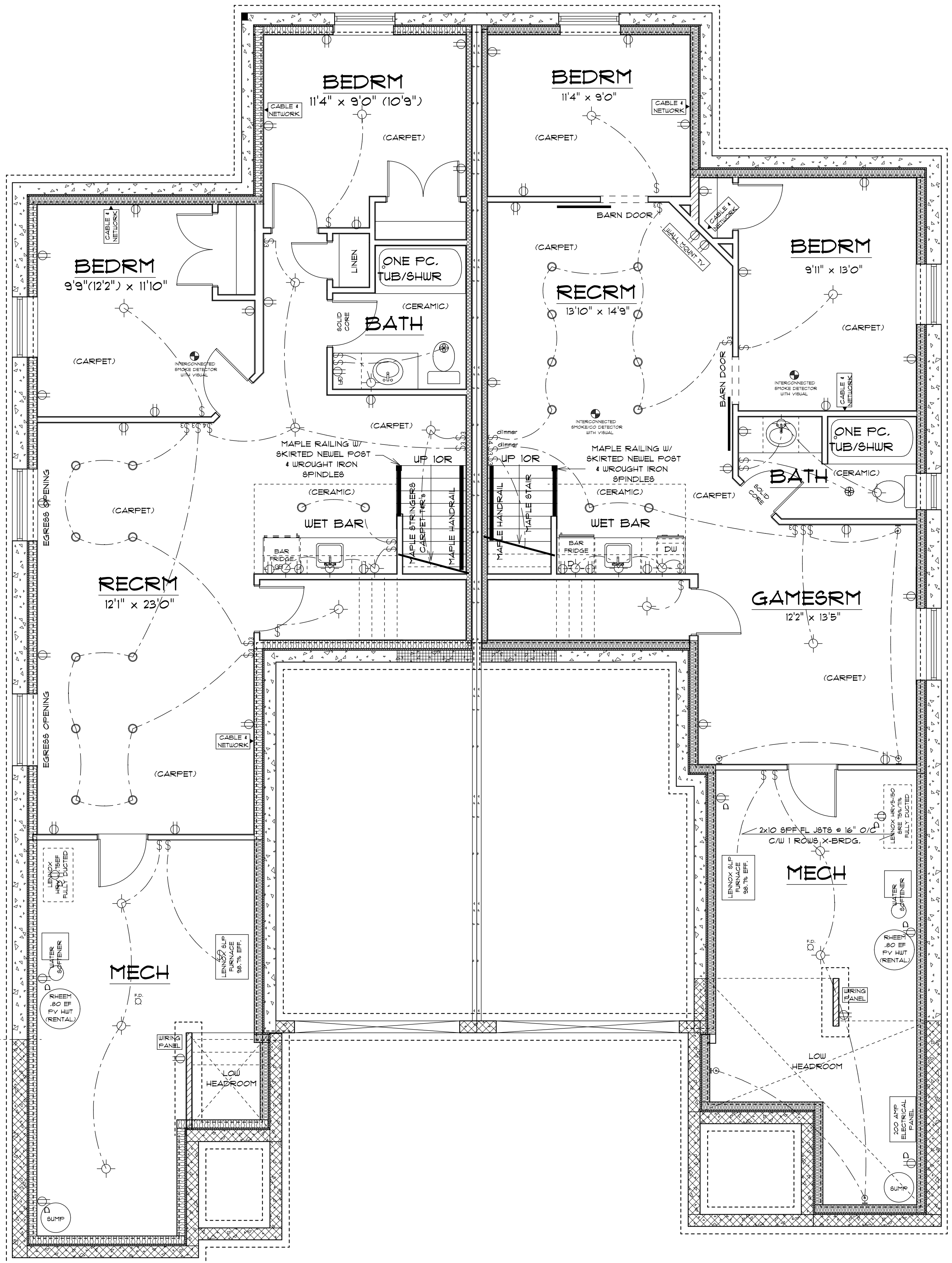
SEMI DETACHED RESIDENCE (868 SQ FT.) BASEMENT FLOOR PLAN EMERALD HOMES LTD.
